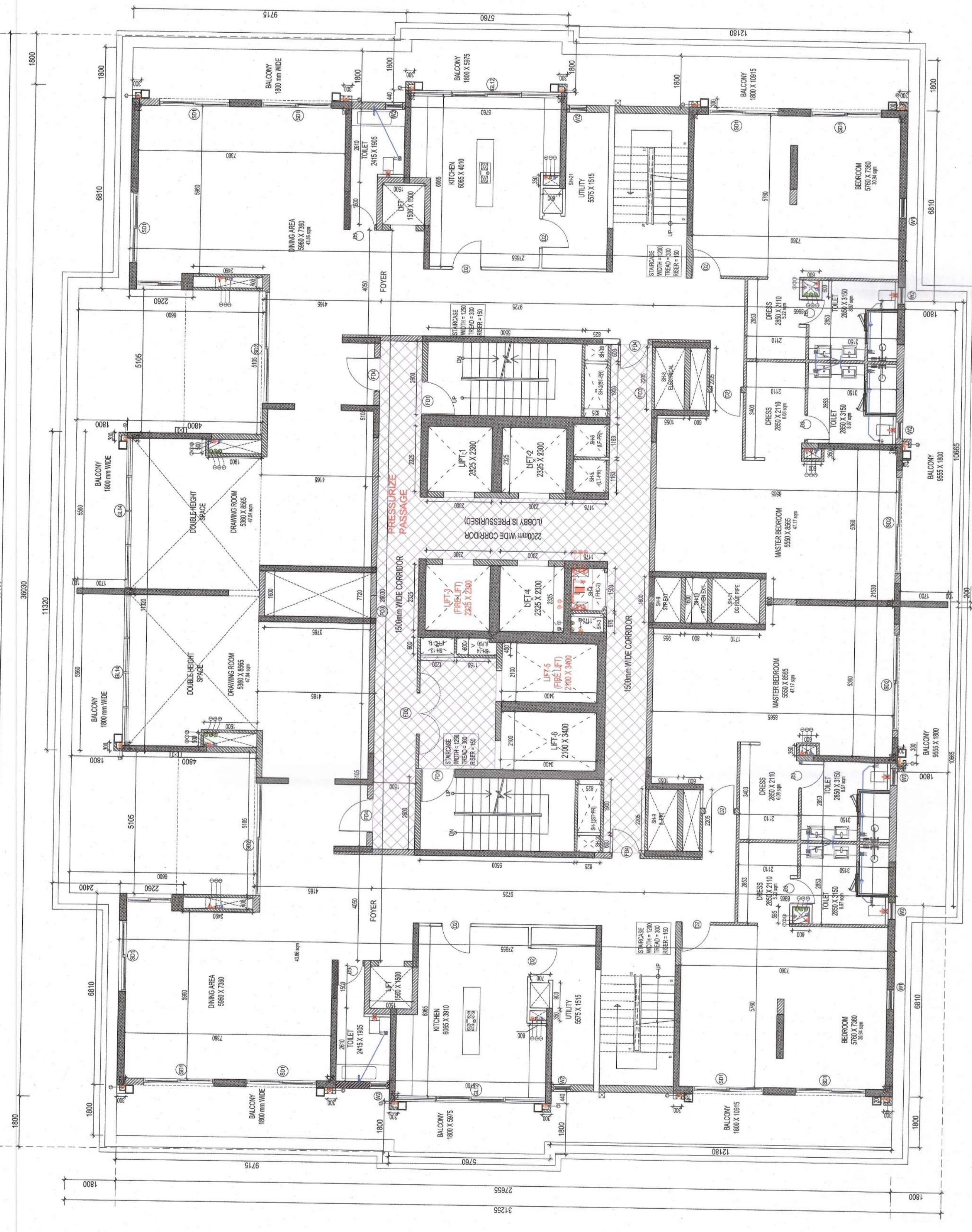
LOWER PENTHOUSE PLAN SCALE 1:100 F.F.L AT +100.000
