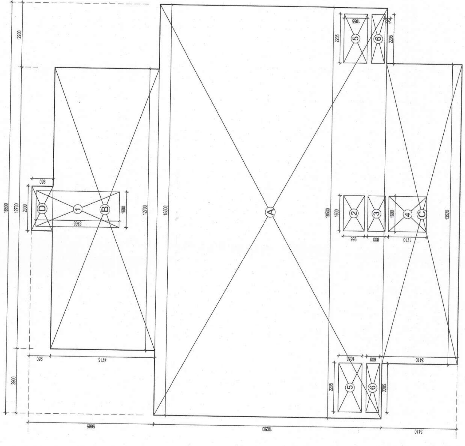
MUMTY & MACHINE ROOF PLAN SCALE 1:100
